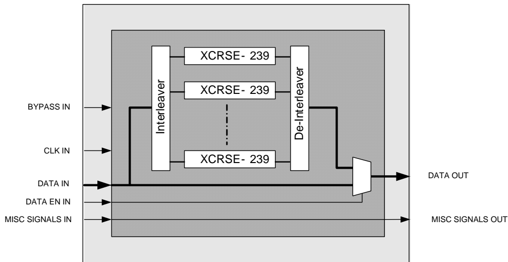
XCO2FECE Block Diagram
